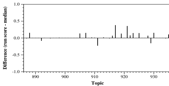
Per-topic difference from median nDCG@5 for Wikification runs
