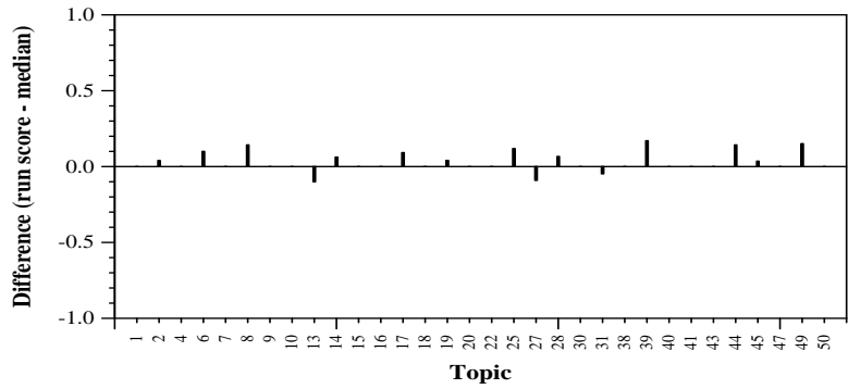
Per-topic difference from median R-precision using binary.incorrect qrels
