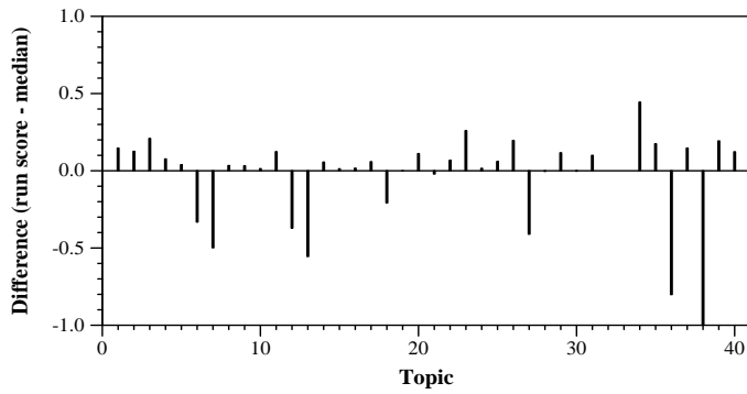
Per-topic difference from median infNDCG for Clinical Trials runs
