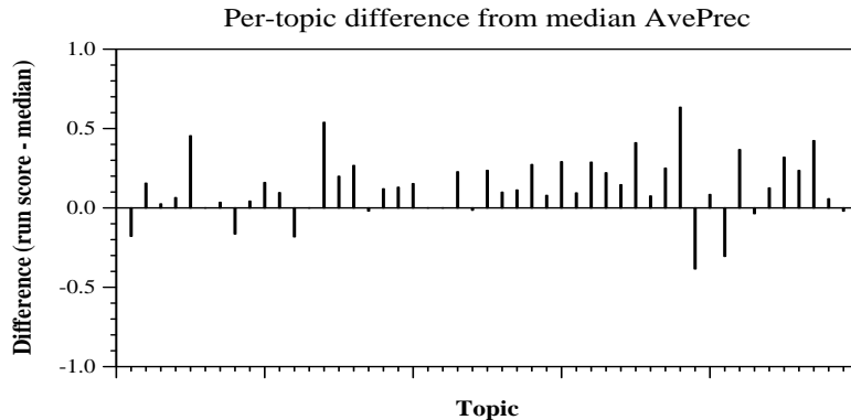
Per-topic difference from median NDCG@10
