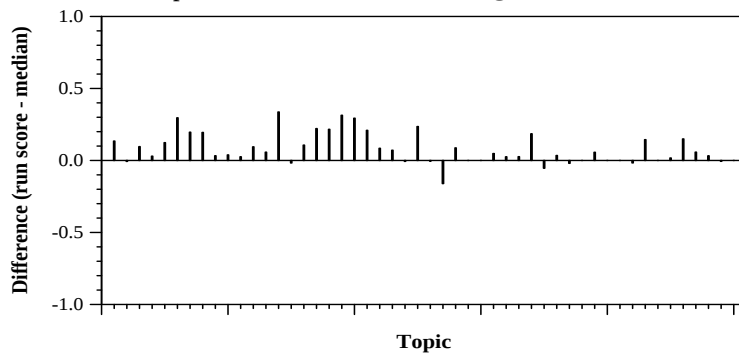
Per-topic difference from median NDCG for Feedback runs
