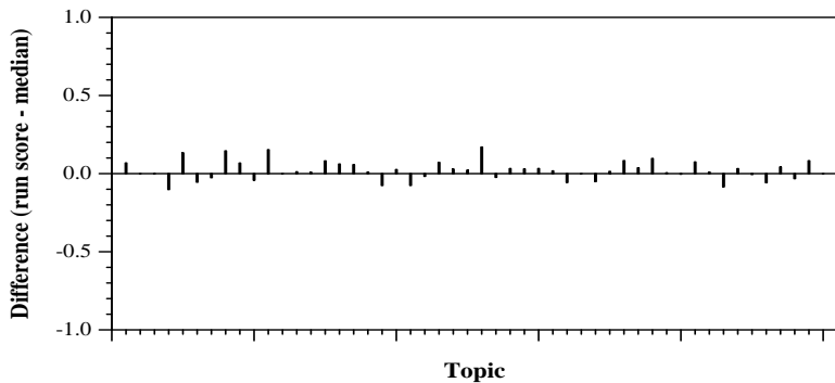
Per-topic difference from median AP for Manual runs
