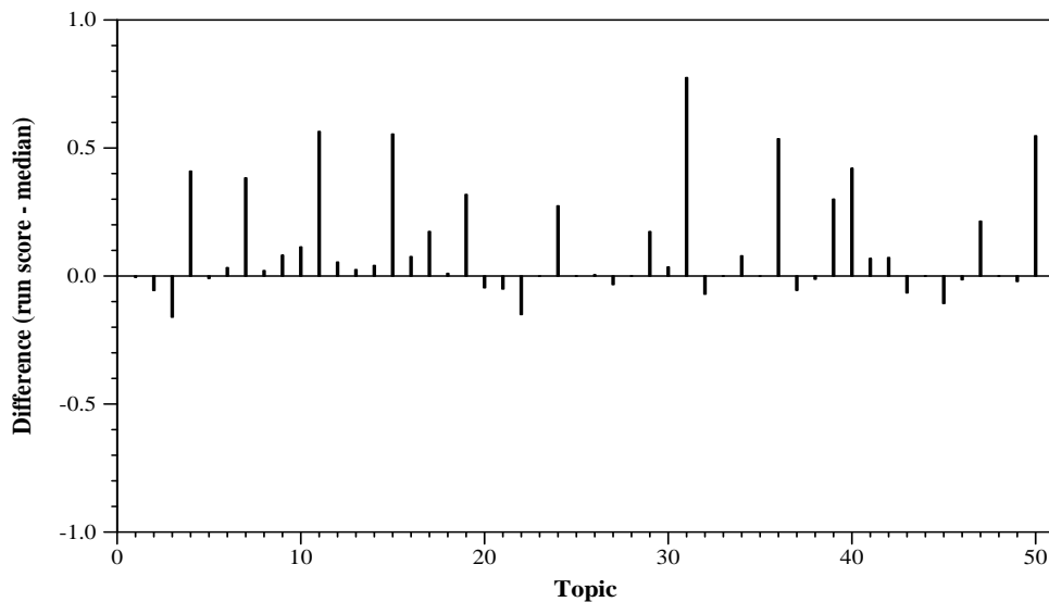
Per-topic difference from median alpha-nDCG@10
