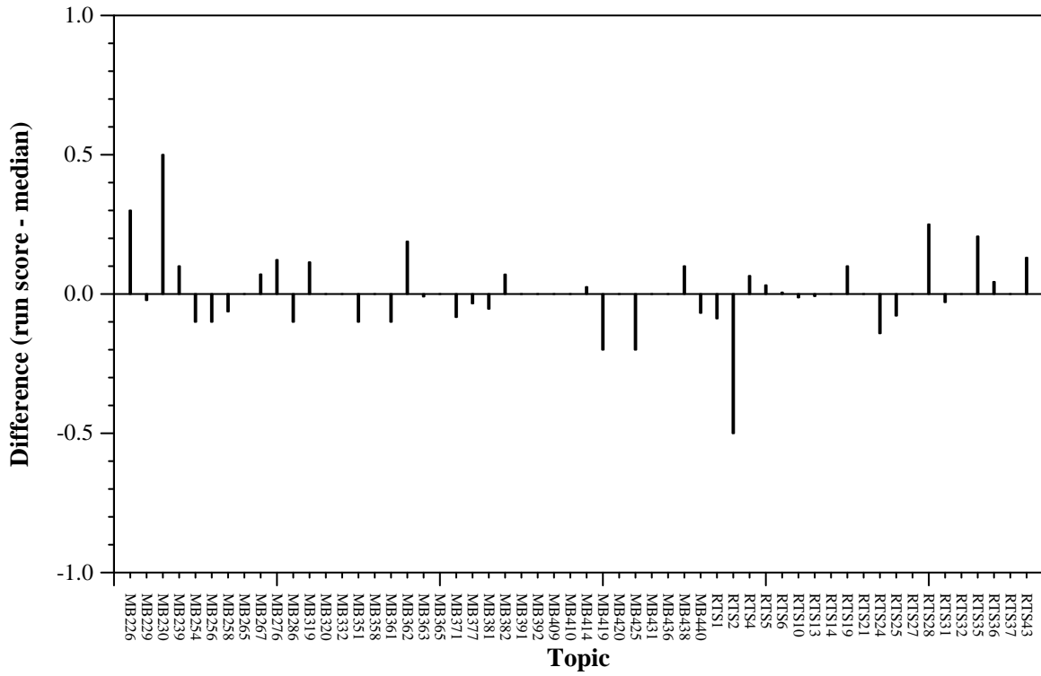
Per-topic difference from median nDCG1
