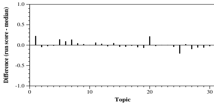
Per-topic difference from median infNDCG for Manual runs
