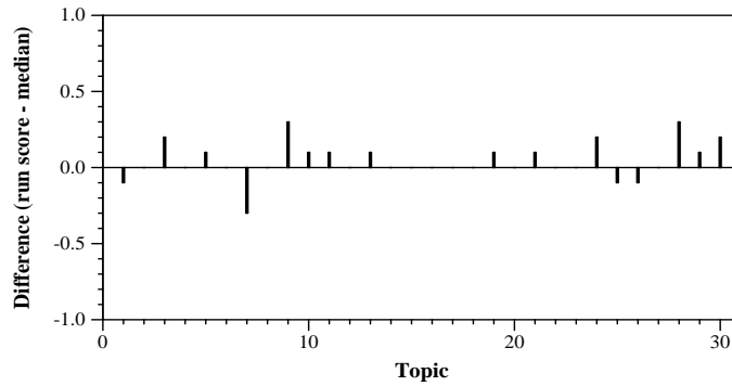
Per-topic difference from median P@10 for Automatic, Summary runs
