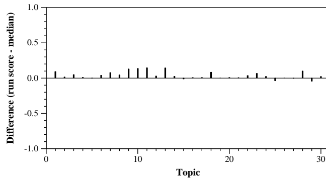
Per-topic difference from median infNDCG for Automatic, Summary runs
