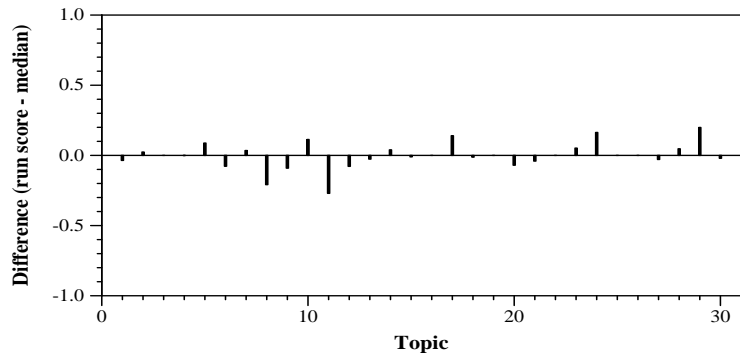
Per-topic difference from median infNDCG for Manual runs
