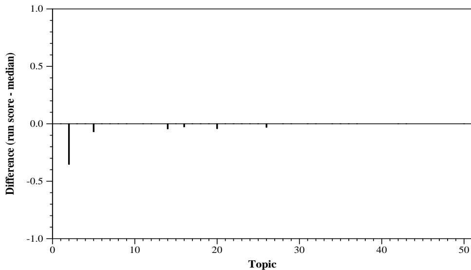
Difference from median ndcg@10 per topic
