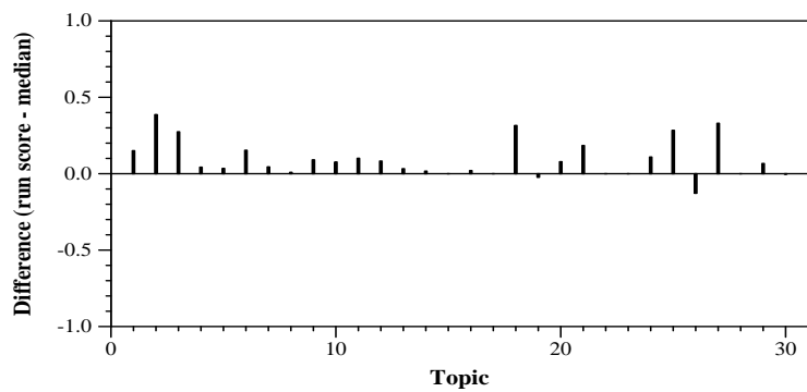
Difference from median infNDCG for manual runs per topic
