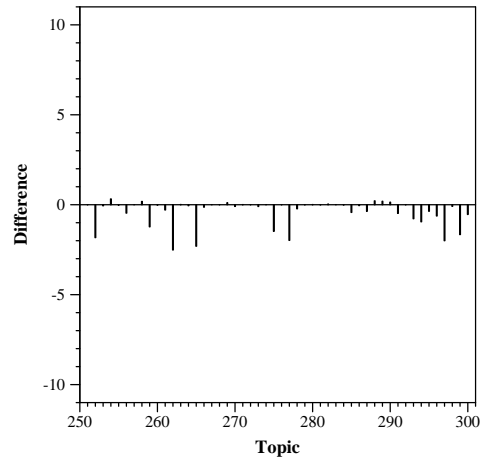
alpha=5,baseline=rm
