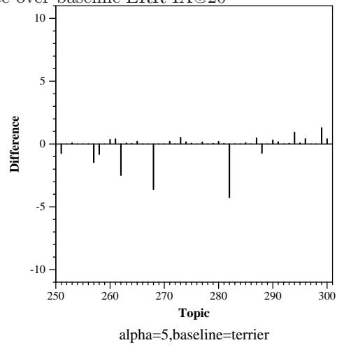
Difference from median for difference-over-baseline ERR-IA@20
