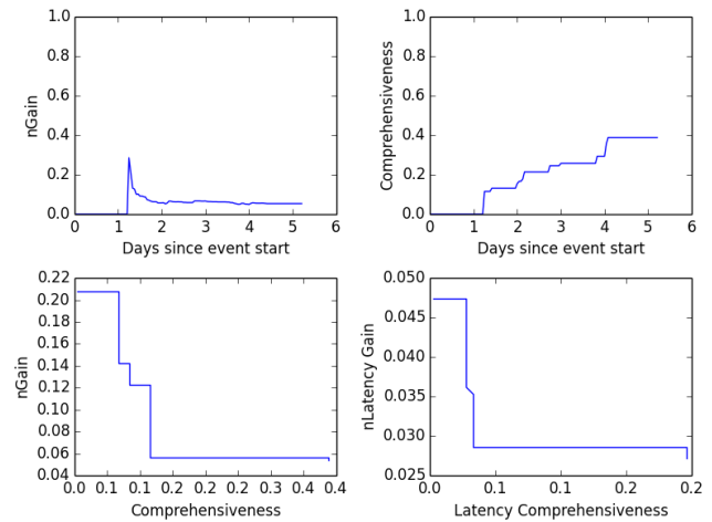
(b) Query 14
