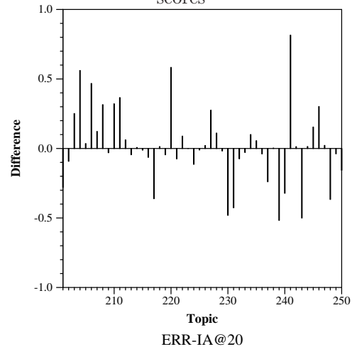
Difference from median for ERR-IA@20 scores
