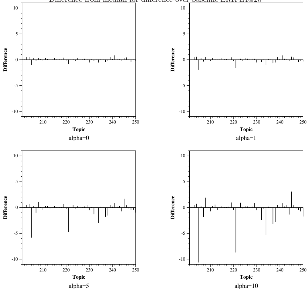
Difference from median for difference-over-baseline ERR-IA@20
