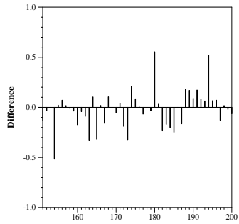
Difference from median \alpha -nDCG@20 per topic
