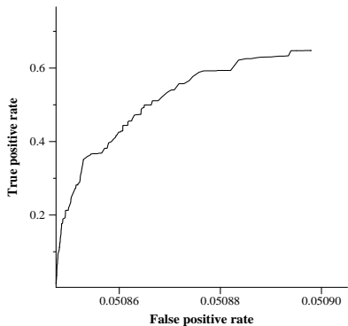
average ROC curve for uwcmb12NT
