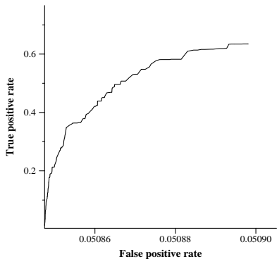
average ROC curve for uwcmb12CP
