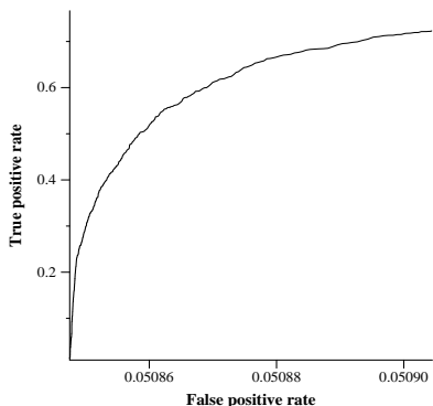
average ROC curve for uwatrrflm
