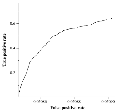
average ROC curve for uwatgclrman
