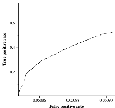
average ROC curve for uwatgclrbase
