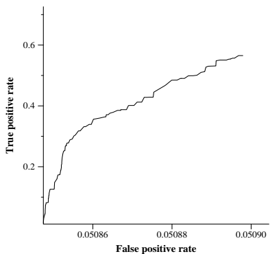
average ROC curve for uiucGSLIS04
