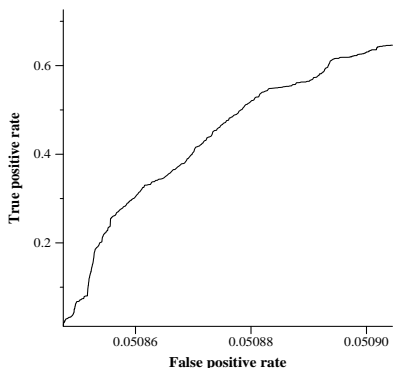
average ROC curve for uiucGSLIS01
