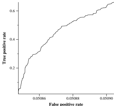
average ROC curve for tsqe
