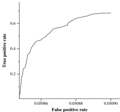
average ROC curve for otM12i
