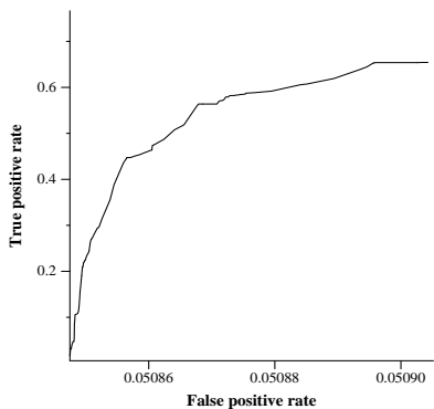
average ROC curve for otM12h
