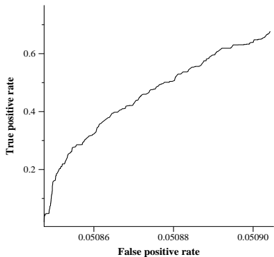
average ROC curve for kobeMHC
