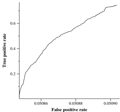
average ROC curve for hitURLrun3
