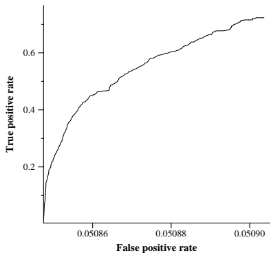
average ROC curve for hitDELMrun2
