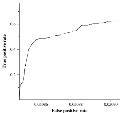
average ROC curve for gucasQuery
