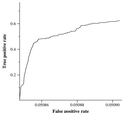
average ROC curve for gucasGenReg
