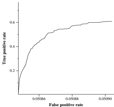
average ROC curve for gucasBasic
