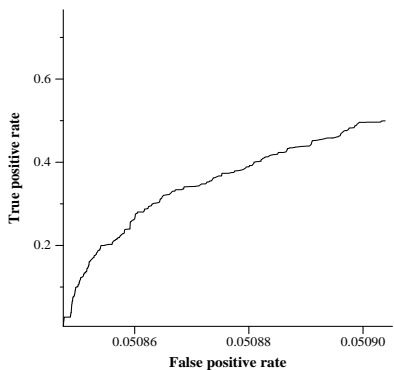
average ROC curve for expansion
