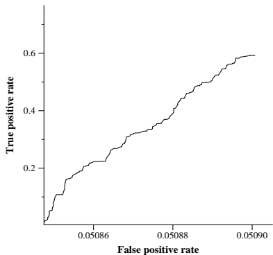
average ROC curve for csiroQE1112
