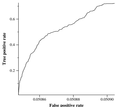
average ROC curve for cmuPrfPhrE
