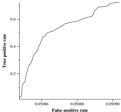
average ROC curve for cmuPrfPhr
