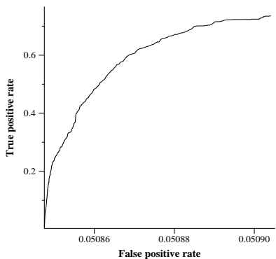
average ROC curve for YORK2
