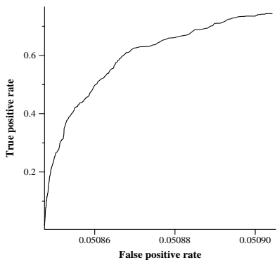
average ROC curve for YORK1
