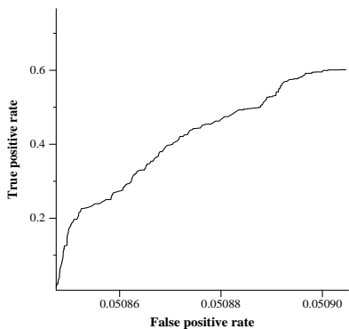
average ROC curve for UNCQE
