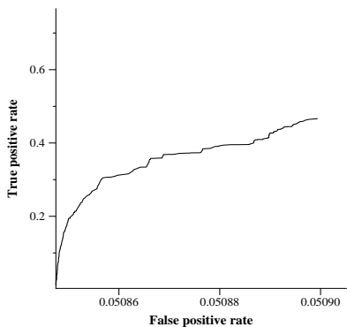
average ROC curve for UDInfoMBTp
