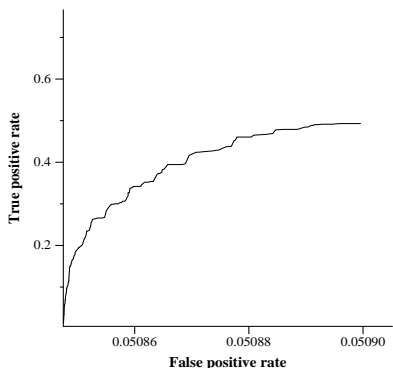
average ROC curve for UDInfoMBIDF
