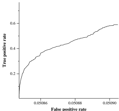
average ROC curve for PKUICST3
