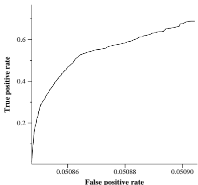
average ROC curve for KLIMLPLL
