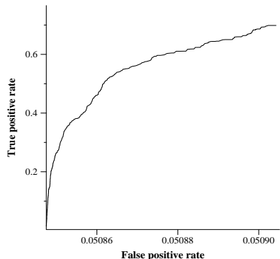
average ROC curve for KLIMLP1
