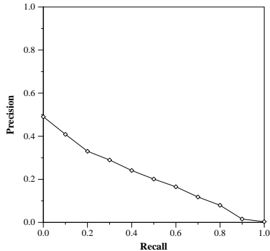
Recall-Precision Curve
