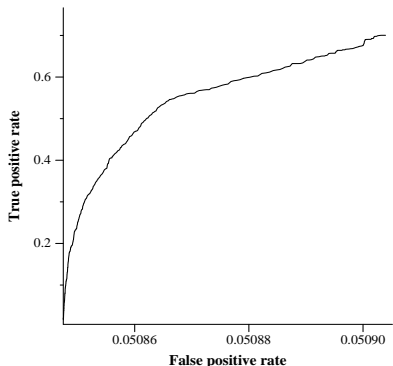
average ROC curve for KLIMLL
