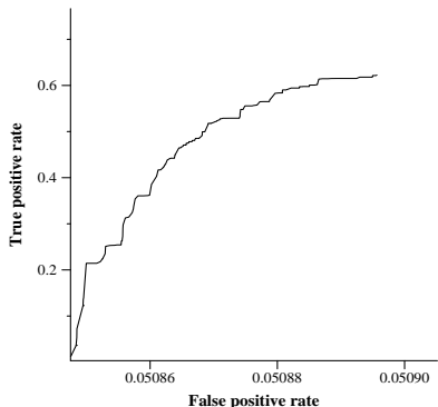
average ROC curve for IRITbnetK
