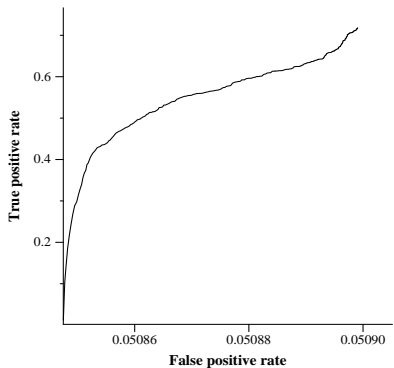
average ROC curve for IBMLTRFuture
